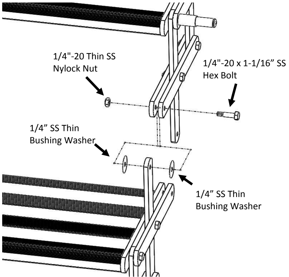
Figure 5.2 Fasten all joints as shown.
