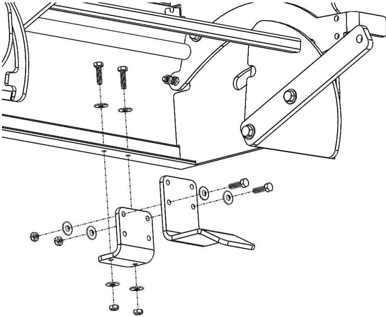
Figure 6.1 4-Step Shelf Bracket Installation
