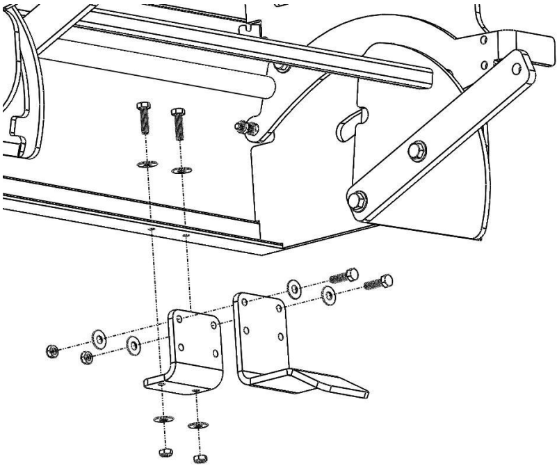
Figure 6.2 5-Step Shelf Bracket Installation
