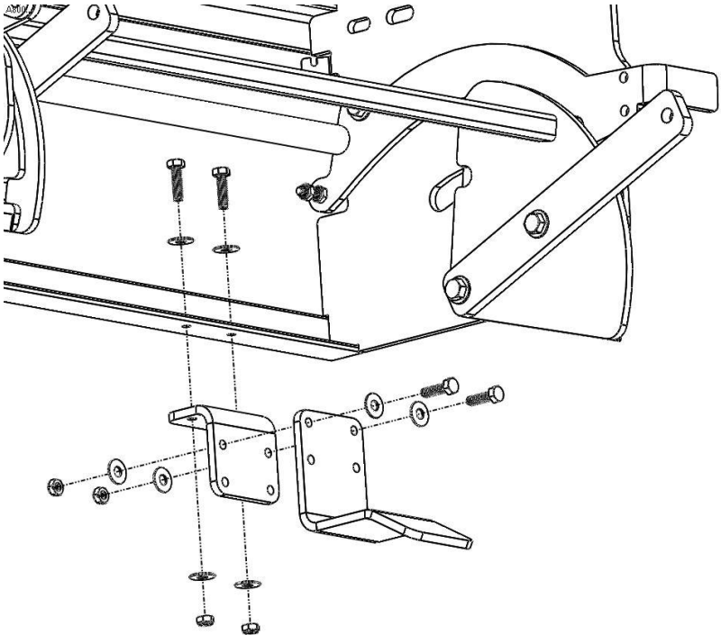
Figure 6.3 6-Step Shelf Bracket Installation
