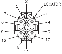
VIEW A-A WIRE INSERTION VIEW
